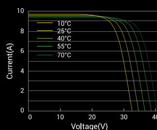
I-V Curve: (A-HCM330)
